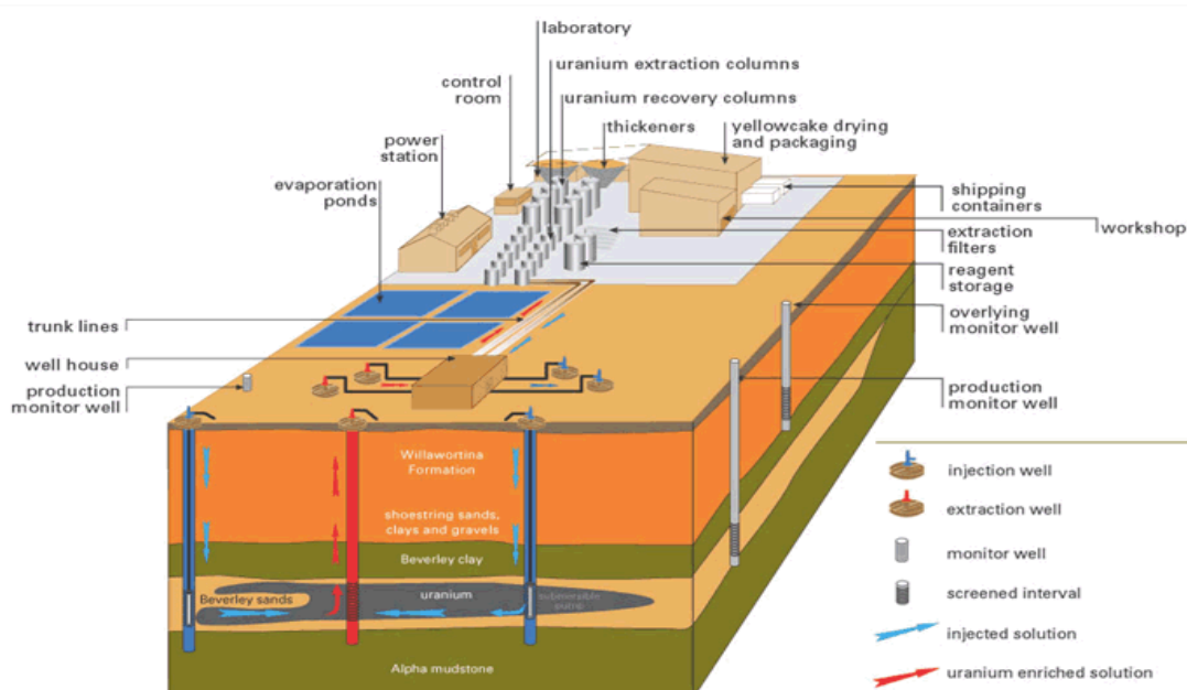
Pictorial representation of ISR uranium mining (Source: World Nuclear Association)
